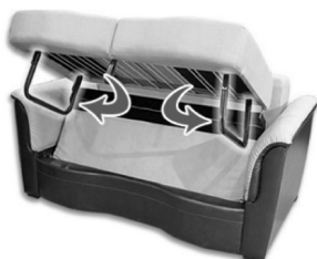
3. While sleeping surface is up, fold out legs. Extend sleeping surface until grounded.
