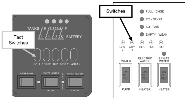
Monitor Panel
