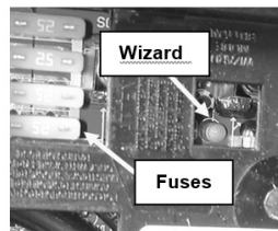
Wizard Button & Reverse Protection Fuses
