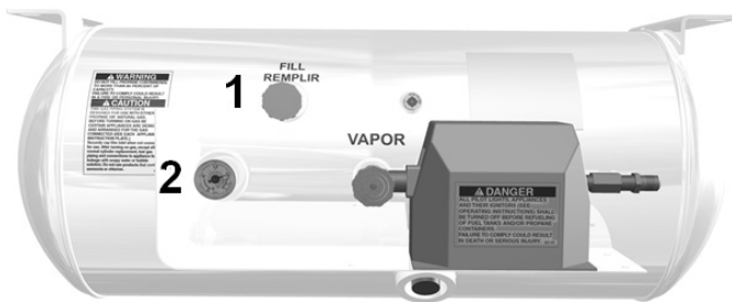
1: Propane fill valve; 2: Propane gauge ASME Tank
