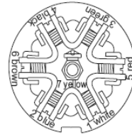
7-way trailer plug Car end, rear view
