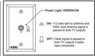
Power Injector
