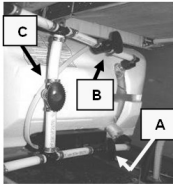
Factory installed water heater bypass
